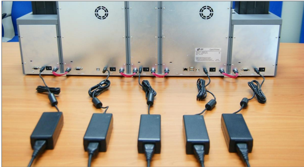
Figure 57 Cable connection of SMART-70 IPHLO
