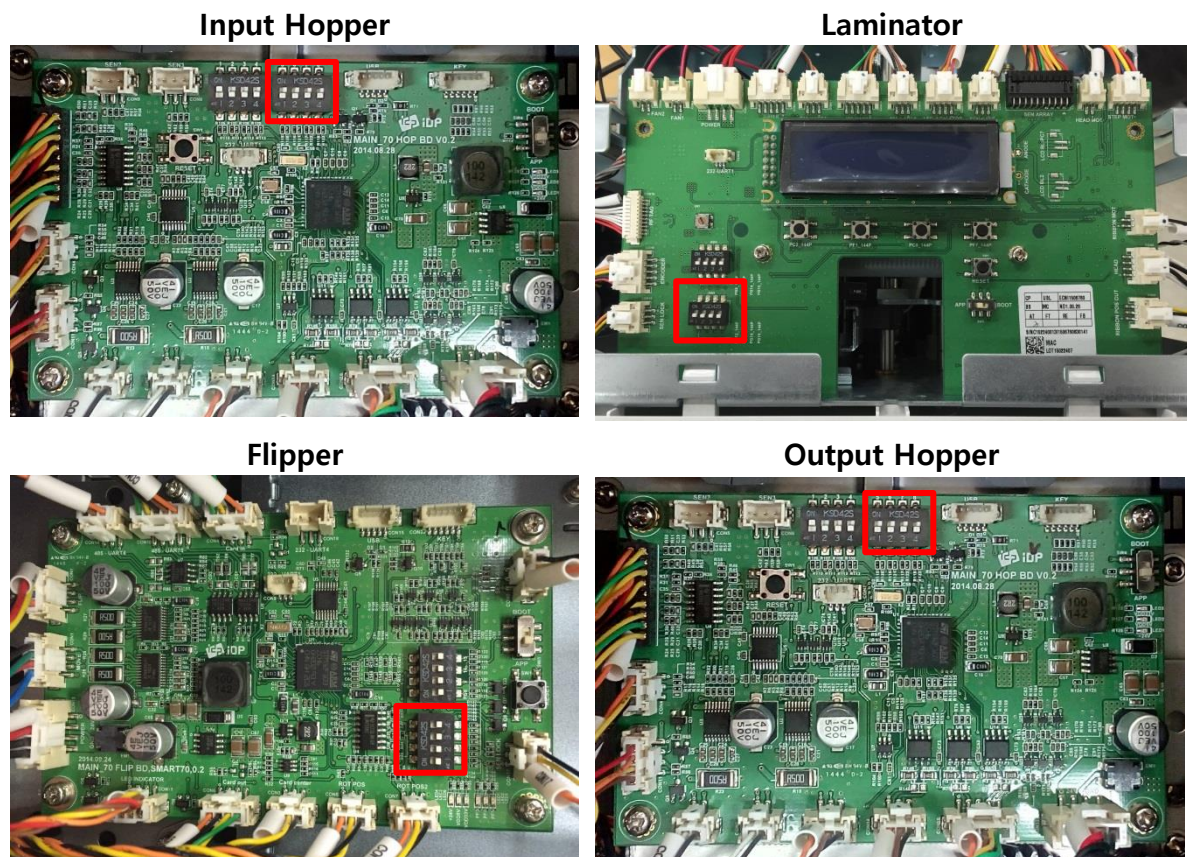
Figure 55 DIP switch location of SMART-70 module
