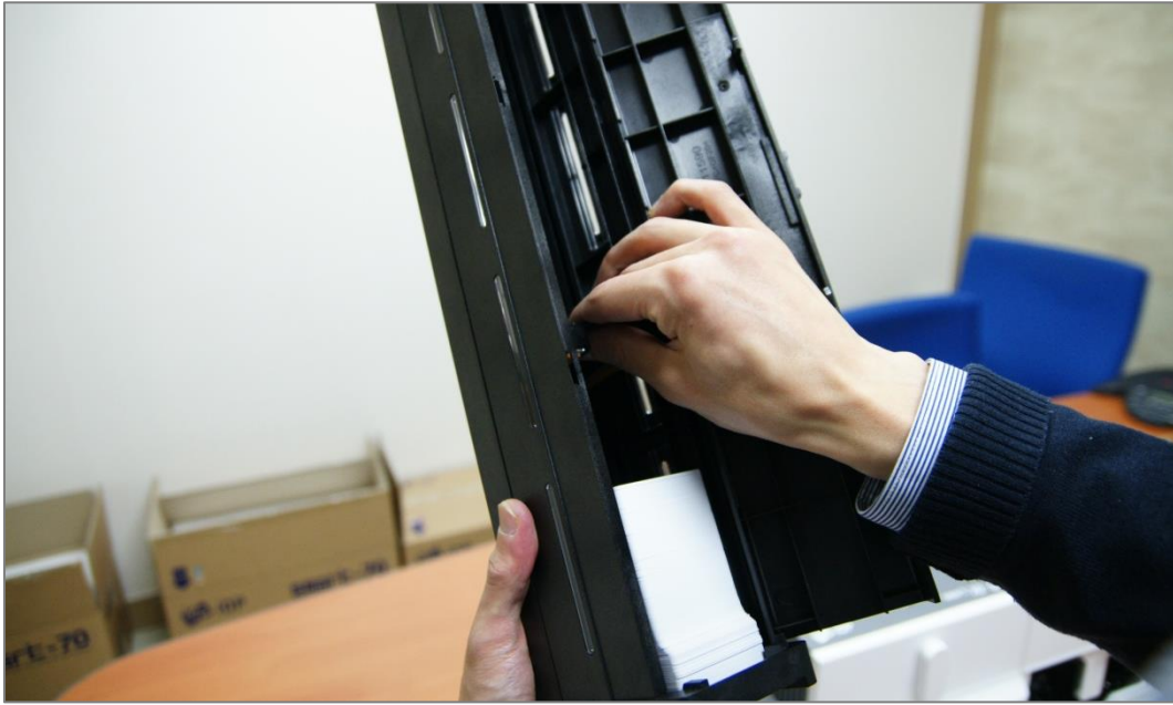
Figure 38 Putting down the card cartridge's weight
