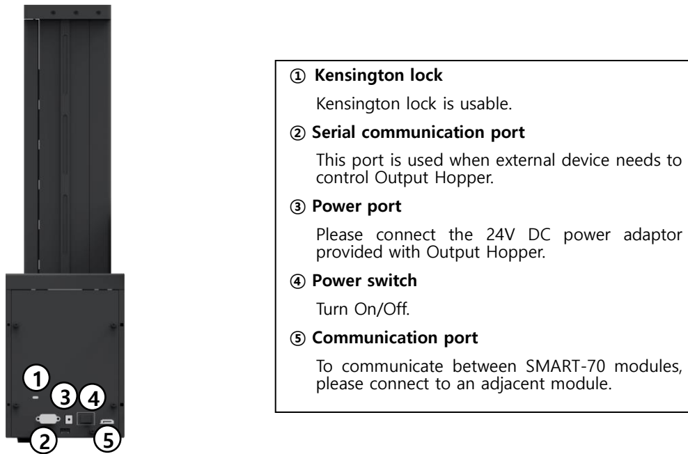
Figure 13 Rear side of Output Hopper
